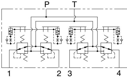
Hydraulic circuit
